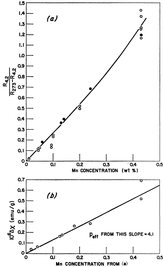
FIG. 1. (a) Resistance ratio as a function of weight percent manganese determined from spectroscopic analysis or quantity of manganese added to the melt. The solid circles represent data from the thesis of W. B. Muir, University of Ottawa. (b) The increase in susceptibility of pure zinc as a function of manganese concentration as determined from the resistance ratio of the alloys measured.
